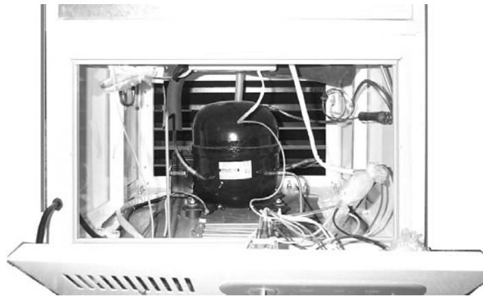
Figure 2 System Access Panel Open
