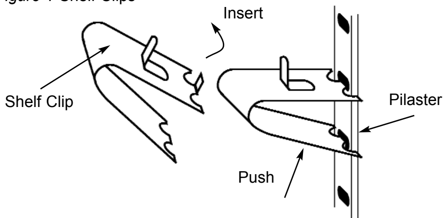
Figure 1 Shelf Clips
